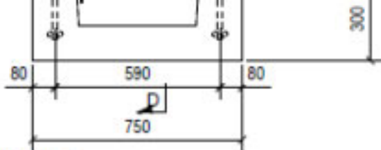
DETAIL - 4 Level 3&5 INTERMEDIATE
