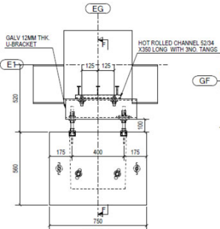
DETAIL - 6 Level GF @ Column
