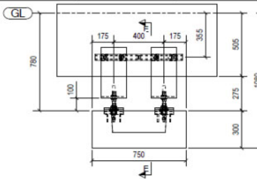
DETAIL - 5 Level 4 INTERMEDIATE
