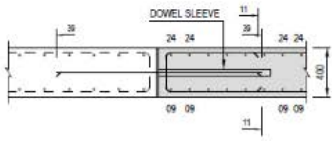
SECTION 7-7 SCALE 1:25
