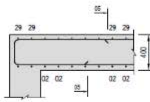
SECTION 6-6 SCALE 1:25
