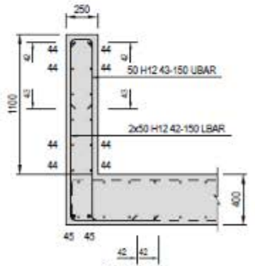
UPSTAND DETAIL A SCALE 1:25
