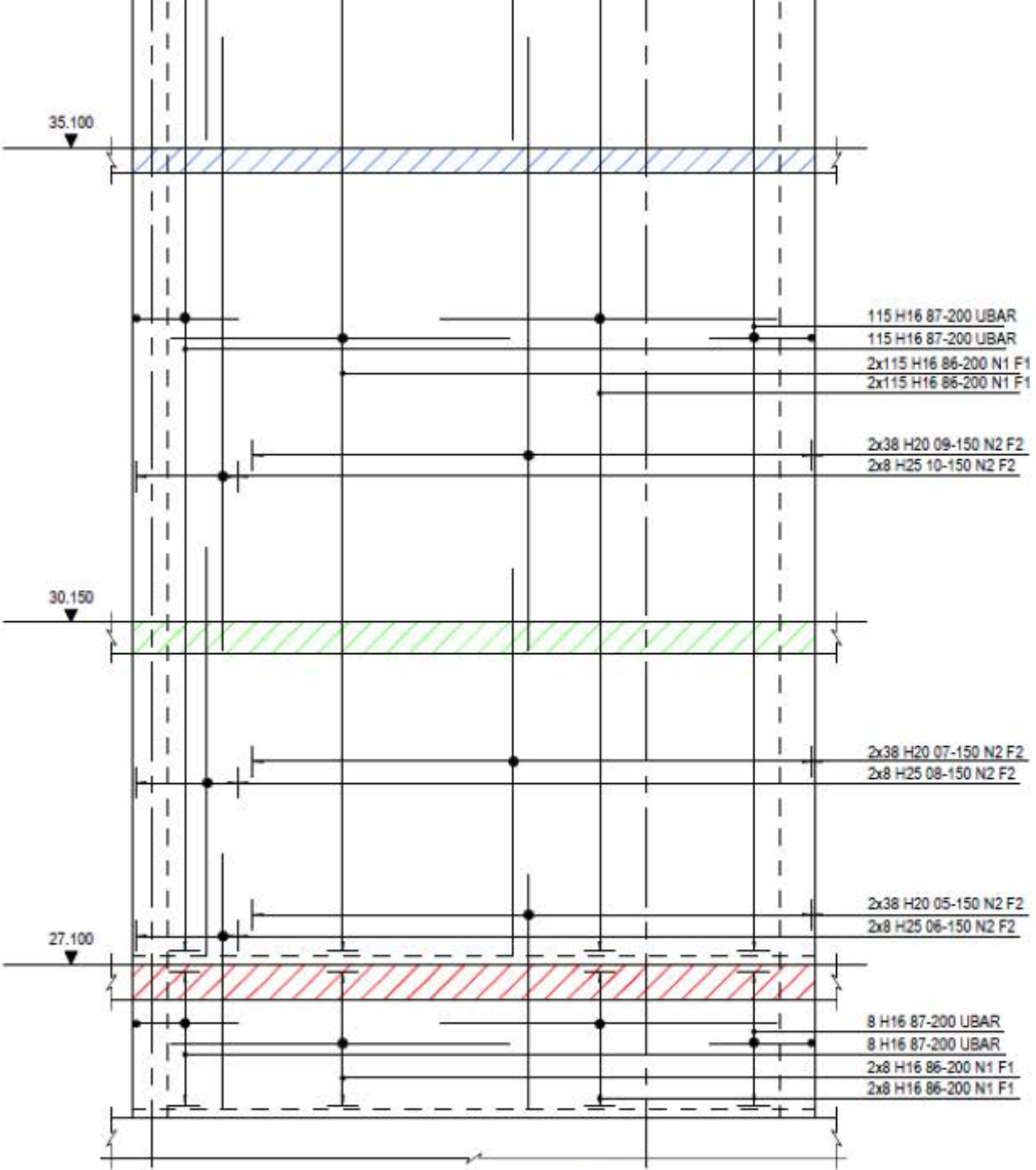
ELEVATION OF CORE WALL 1
