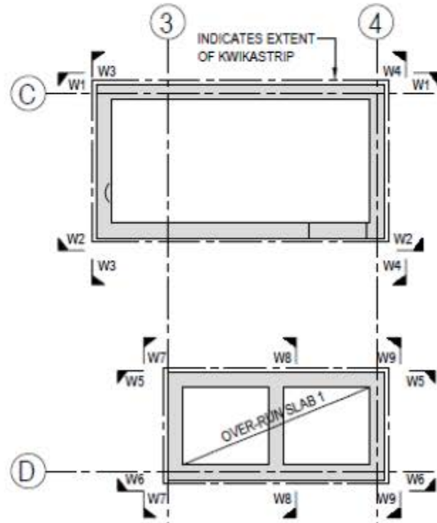
CORE 1 KEYPLAN
