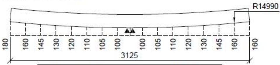
MOULD PROFILE
