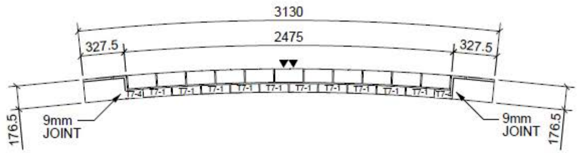
SECTION A - A 1:30
