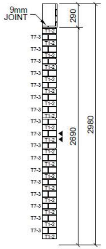
SECTION 2 - 2 1:30
