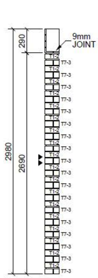
SECTION 1 - 1 1:30
