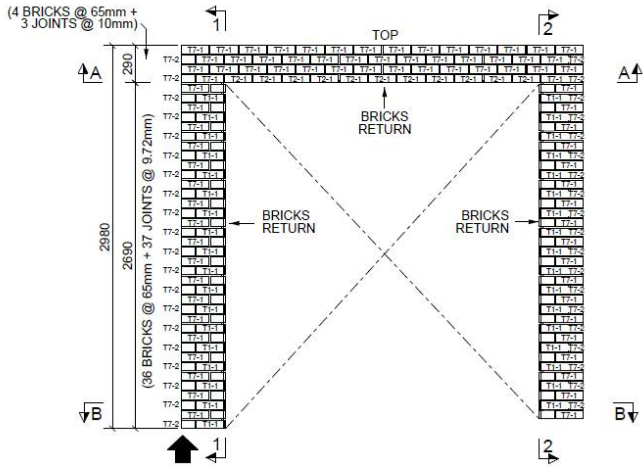
FRONT VIEW 1:30
